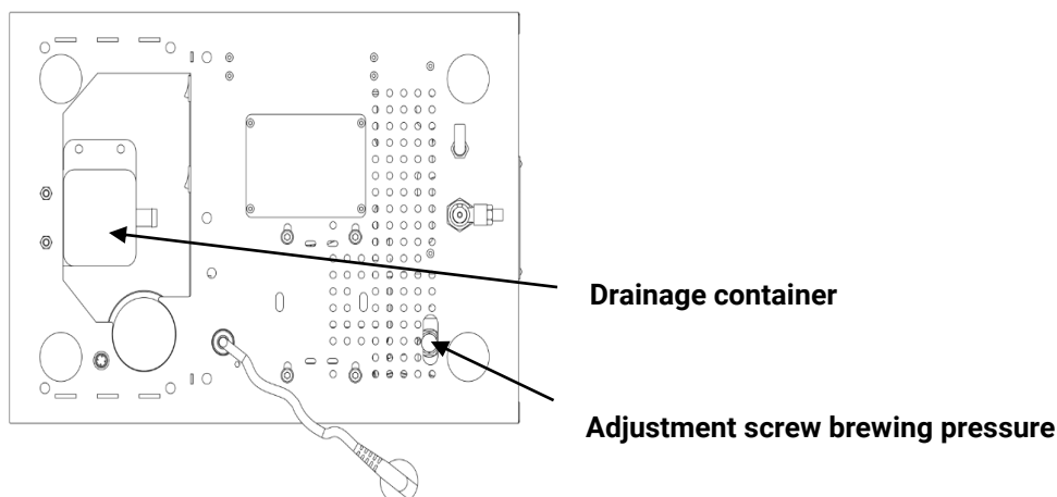
Image 5: Machine bottom
